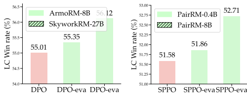
Figure 4: eva scales with quality of reward models , under pointwise RMs w/ DPO ( left ) and pairwise RMs w/ SPPO ( right ). Note SPPO handles general preferences thus requires pairwise RMs, and DPO relies on the Bradley-Terry assumption, for which pointwise RMs are suitable.
