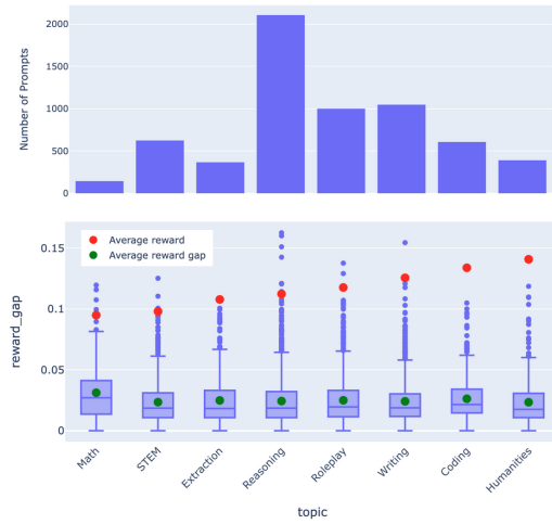
Figure 6: The initial prompt distribution of AlpaEval by bart-large-mnli with 0-shot classification, which is imbalanced. For the reward distribution, the category with lowest average reward has the highest reward gap ( i.e. , the default informativeness proxy), implying the potential to improve.
